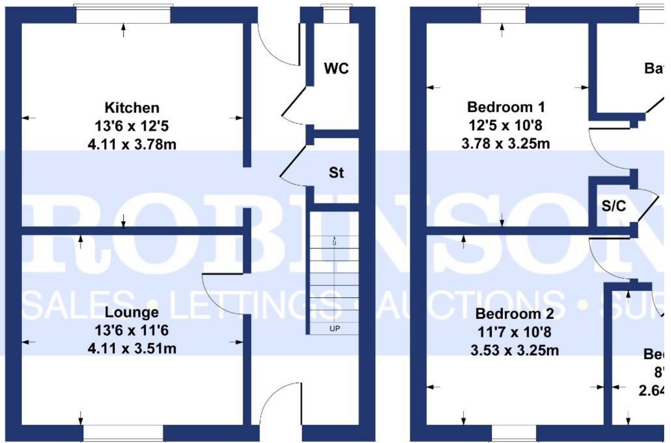
GROUND FLOOR
